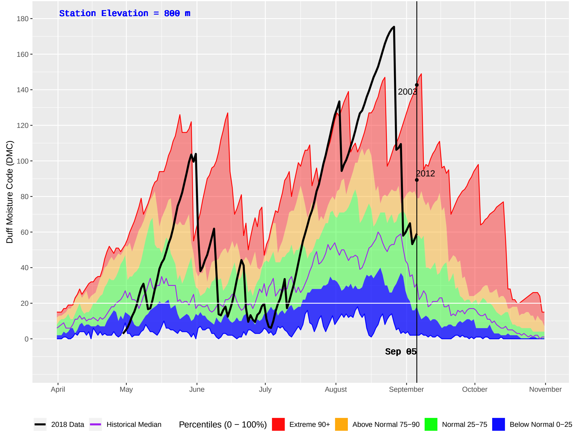
GOLD HILL (379) : Historical (1979–2016) and Current (2018) Daily Duff Moisture Code (DMC)
