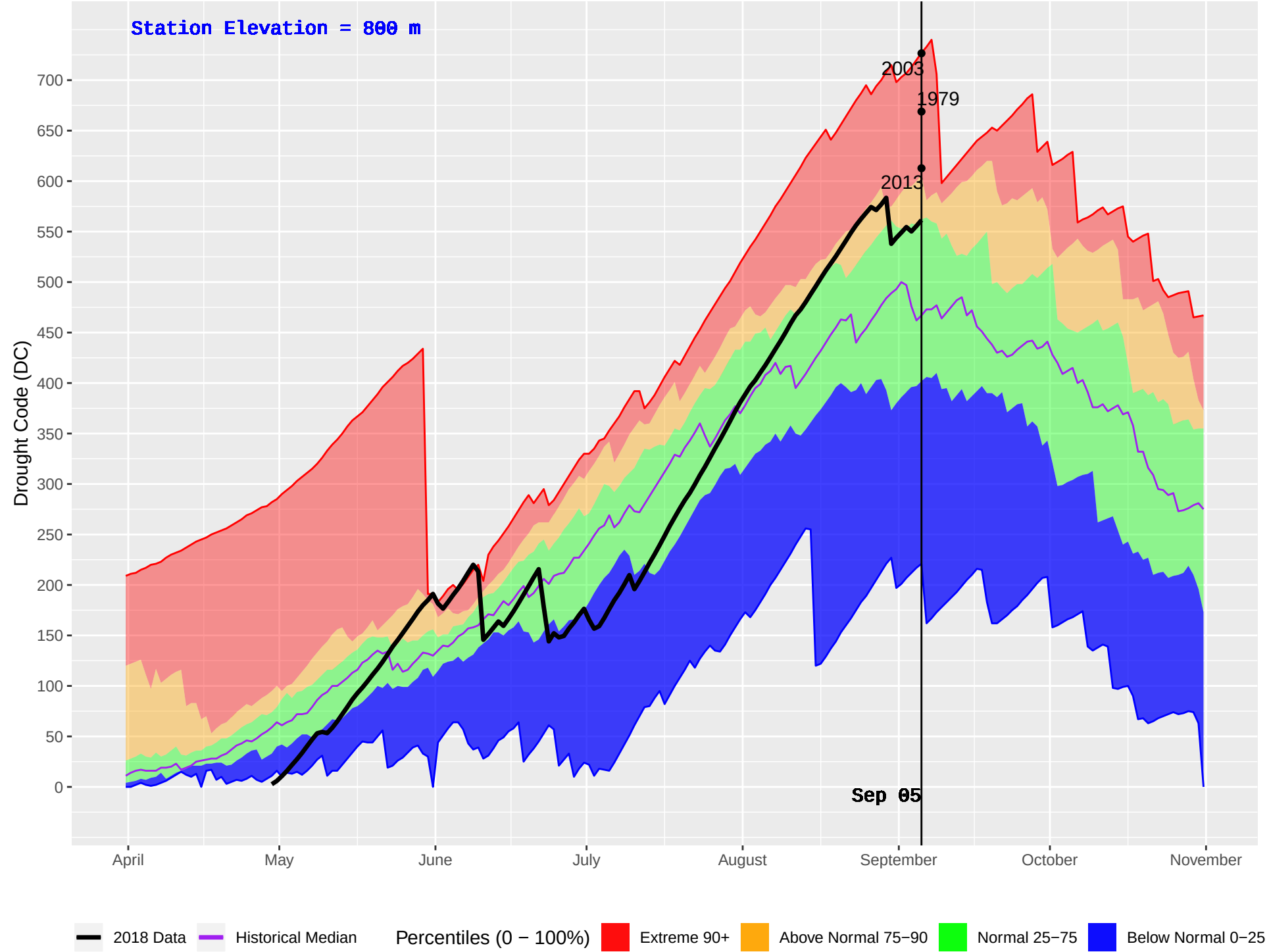
GOLD HILL (379) : Historical (1979–2016) and Current (2018) Daily Drought Code (DC)
