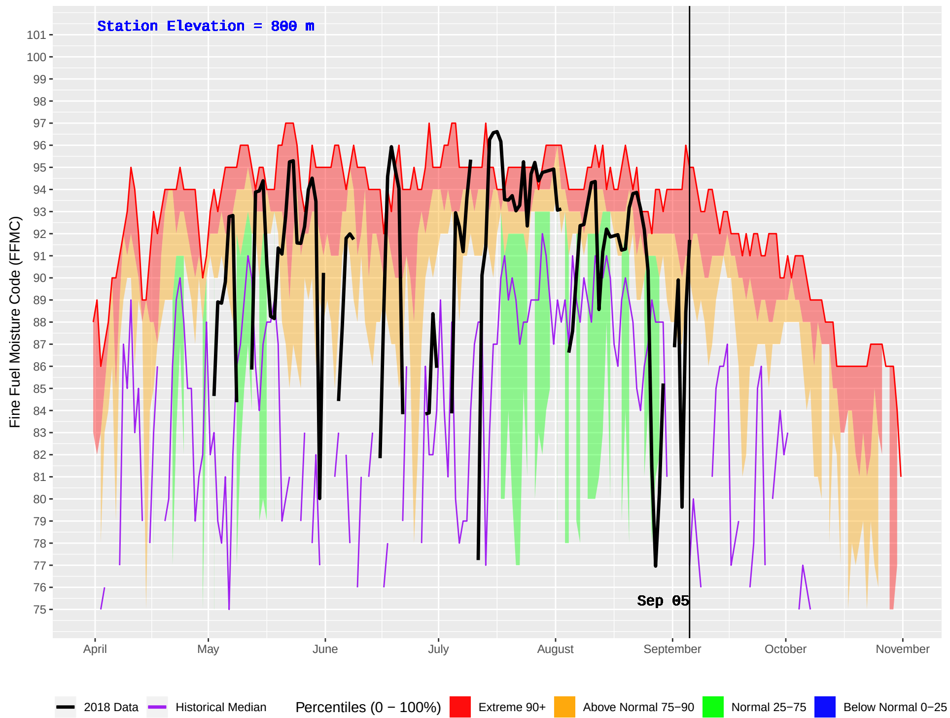
GOLD HILL (379) : Historical (1979–2016) and Current (2018) Daily Fine Fuel Moisture Code (FFMC)
