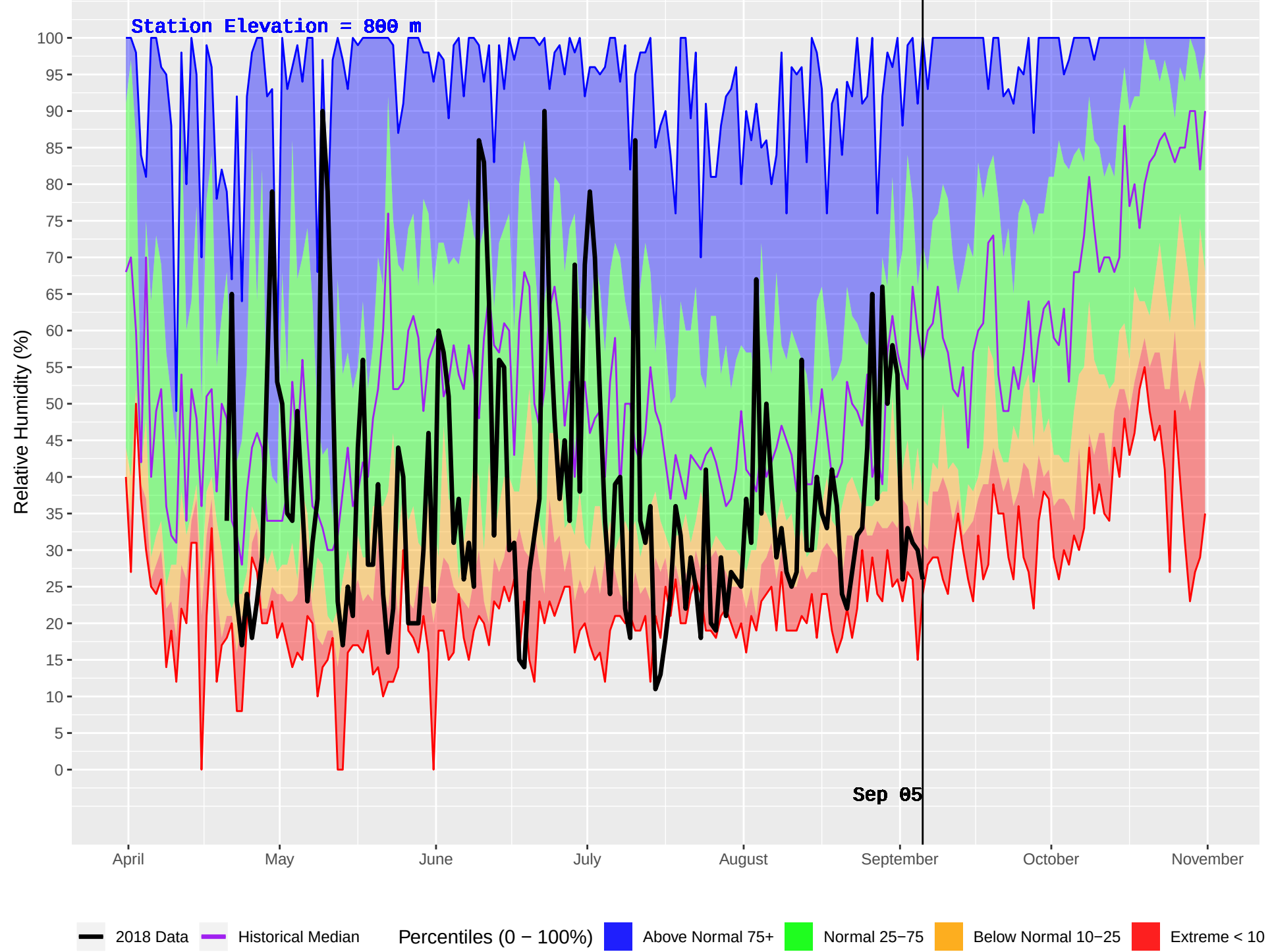
GOLD HILL (379) : Historical (1979–2016) and Current (2018) Daily Relative Humidity
