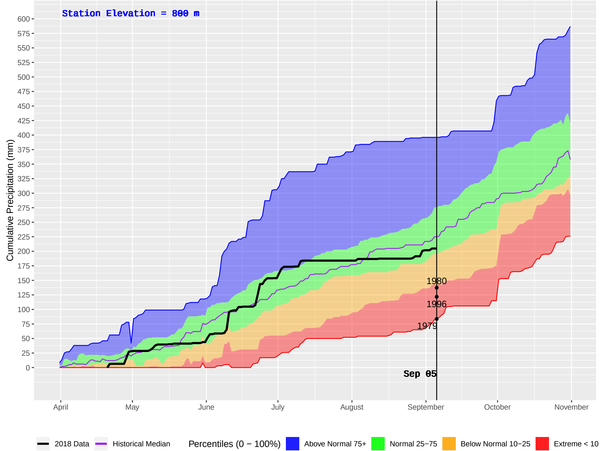
GOLD HILL (379) : Historical (1979–2016) and Current (2018) Daily Cumulative Precipitation
